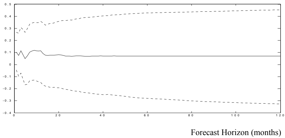
b. Correlation between first and third moments 86Y Differenced VAR
