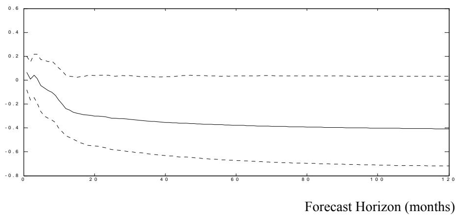
c. Correlation between first and fourth moments 86Y Differenced VAR
